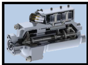
C-130J Fuel Flow Transmitter (cut away) P/N 9-127-67
